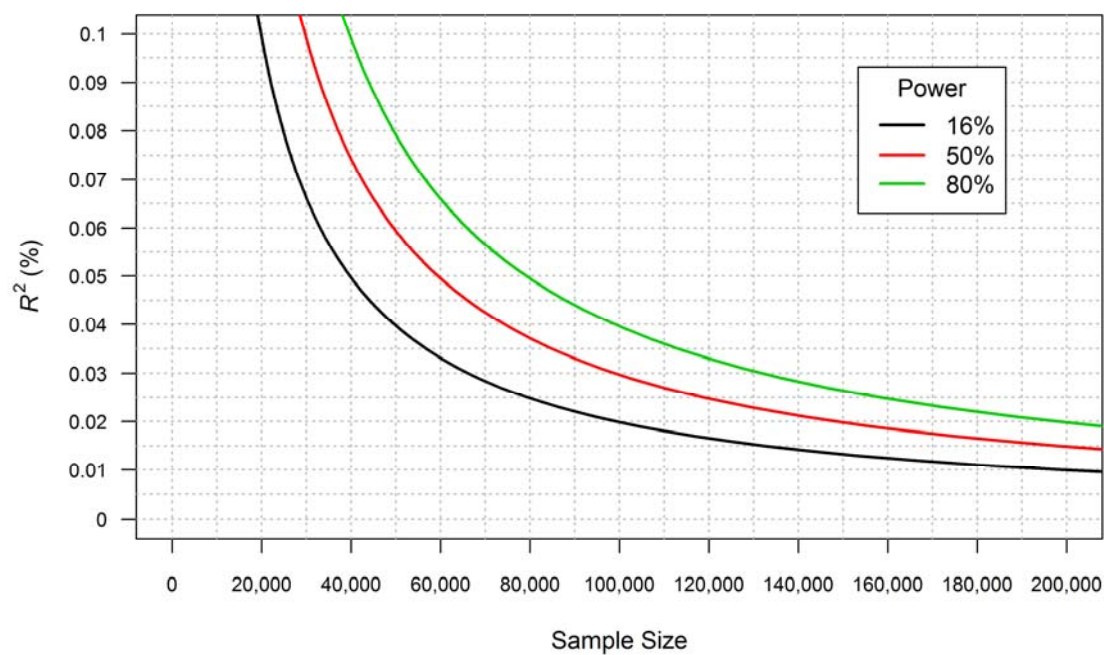
Figure S22. An illustration of the tradeoff between a GWAS on a distal phenotype in a larger sample against a GWAS on the endophenotype in a smaller sample. The y -axis shows effect sizes in terms of the population R^2 from the regression of the phenotype on the single SNP, ranging from 0 to 0.1% in increments of 0.01% (one-hundredth of one percent). The x -axis is the sample size. In these calculations, we assume that the only source of correlation between the SNP and Y is the effect of the SNP on the endophenotype of interest. Each curve graphs the locus of effect-size/sample-size pairs that gives a given level of power to detect the association at p=5\times 10^{-8} .
